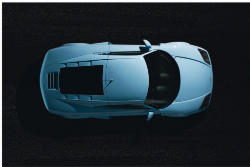
junction eleven
