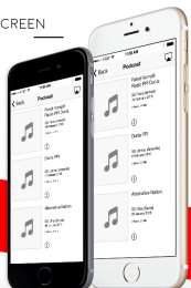
PODCAST SCREEN
