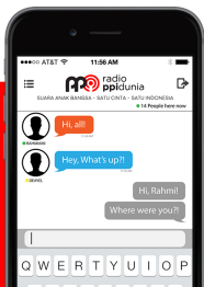
CHATBOX SCREEN
